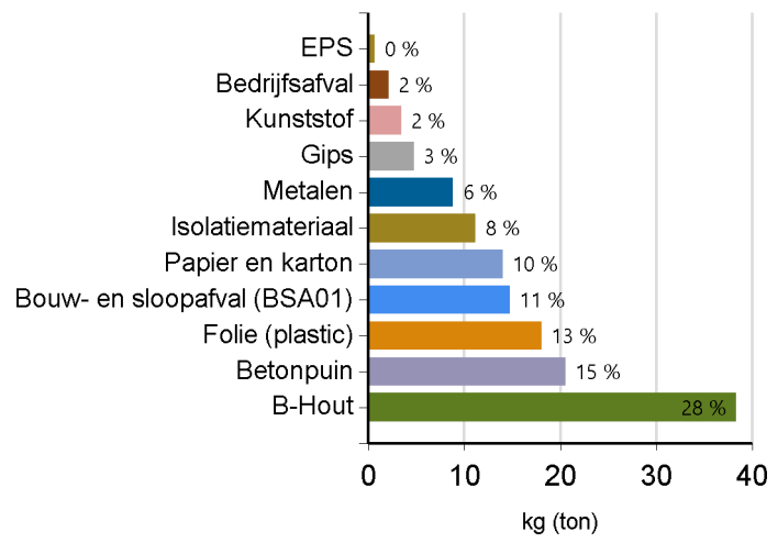
Scheidingspercentage (kg)
